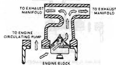
COOLANT FLOW THROUGH THERMOSTAT HOUSING WITH THERMOSTAT OPEN
