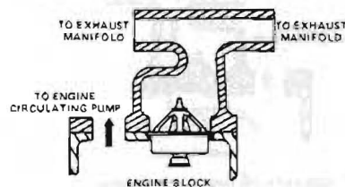
COOLANT FLOW THROUGH THERMOSTAT HOUSING WITH THERMOSTAT CLOSED
