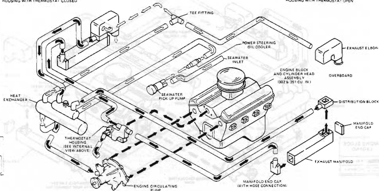
COOLANT FLOW THROUGH THERMOSTAT HOUSING WITH THERMOSTAT CLOSED
