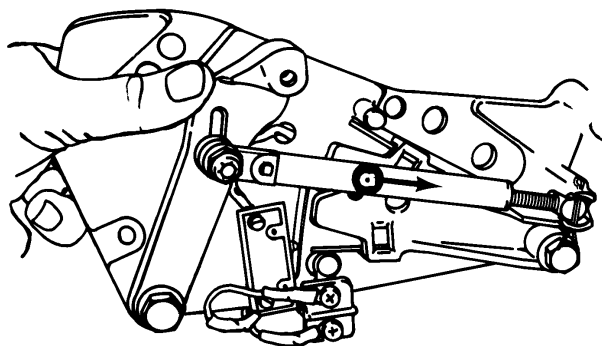
a - Drive Unit Shift Cable - Push In
