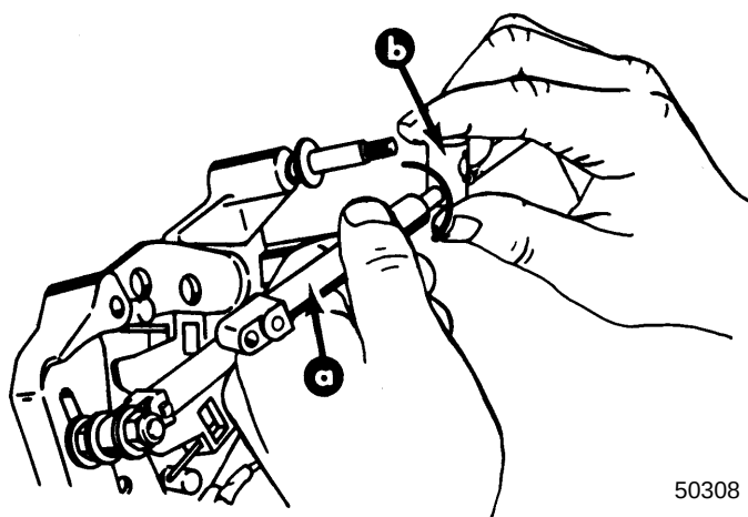
a - End Guide b - Brass Barrel
